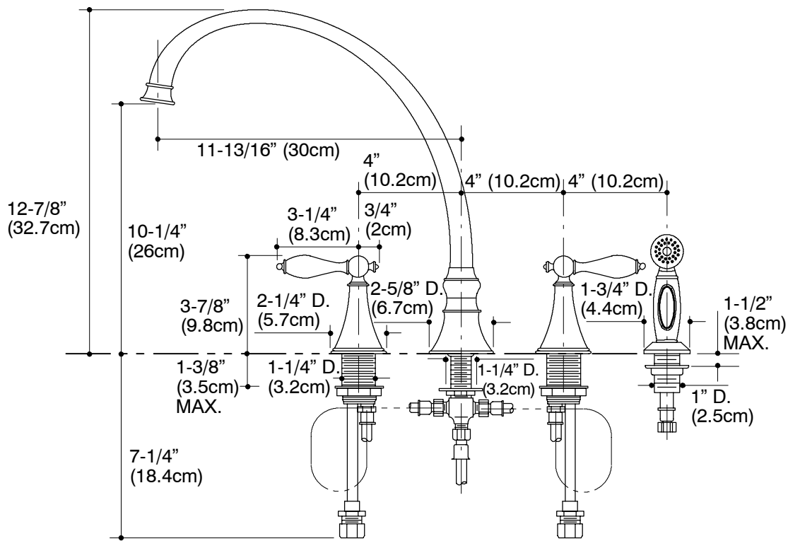
PRODUCT DIAGRAM
